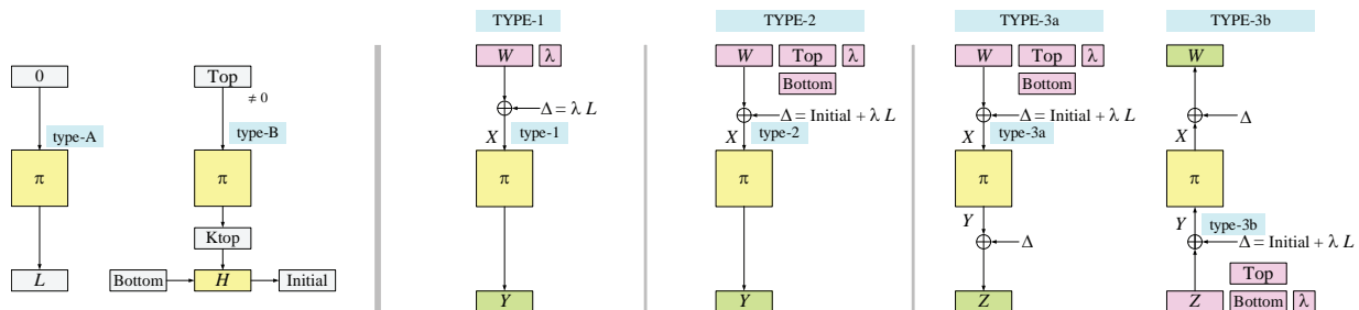
Figure 11: The TW construction. The adversary’s queries (TYPE 1, 2, 3a, 3b) result in internal queries that are either direct (type 1, 2, 3a, 3b) or indirect (type A, B). The proof of Lemma 3 hinges on establishing the rarity of nontrivial collisions among the inputs or outputs of \pi .
